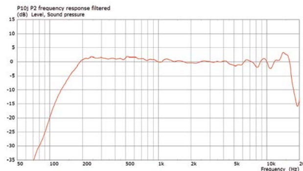
Frequenzgang (processed)
