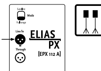
Anschluss-Schema Fullrange-Setup
